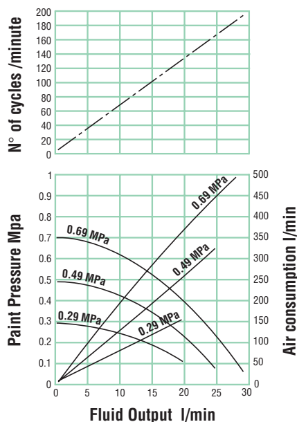
DPS 120-B Performance Curve
